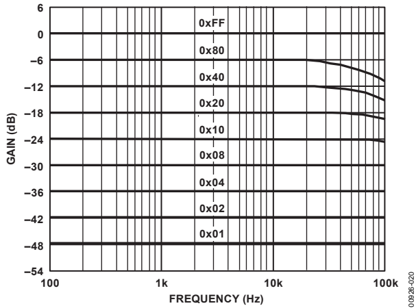
Figure 20. AD5242 100 k \Omega Gain vs. Frequency vs. Code
