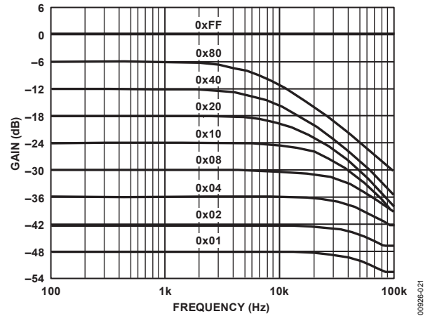
Figure 21. AD5242 1 M \Omega Gain vs. Frequency vs. Code
