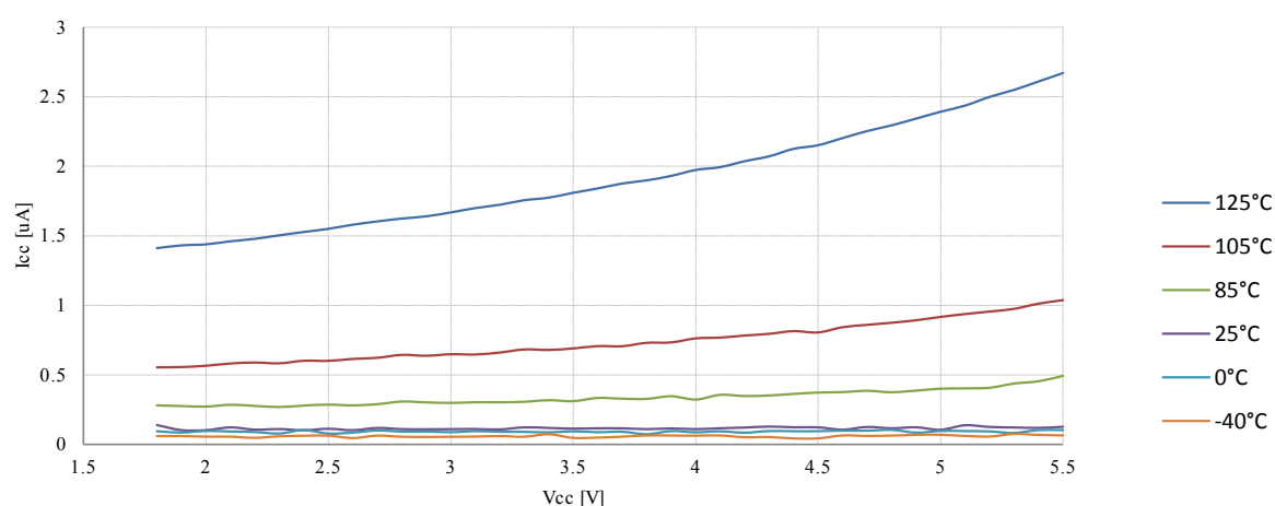
Figure 23-11. Power-down Supply Current vs. V_{CC} (Watchdog Timer Enabled)
