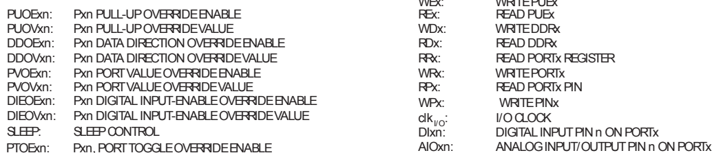
Note: 1. WEx, WRx, WPx, WDr, REx, RRx, RPx, and RDx are common to all pins within the same port. clk I/O and SLEEP are common to all ports. All other signals are unique for each pin.
