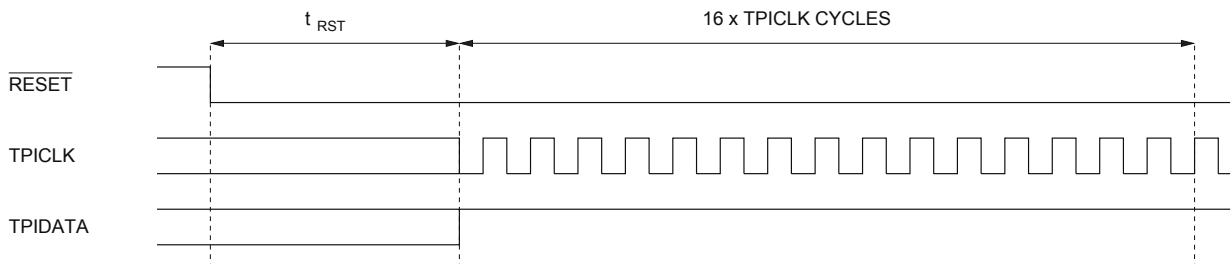
Figure 21-2. Sequence for enabling the Tiny Programming Interface
