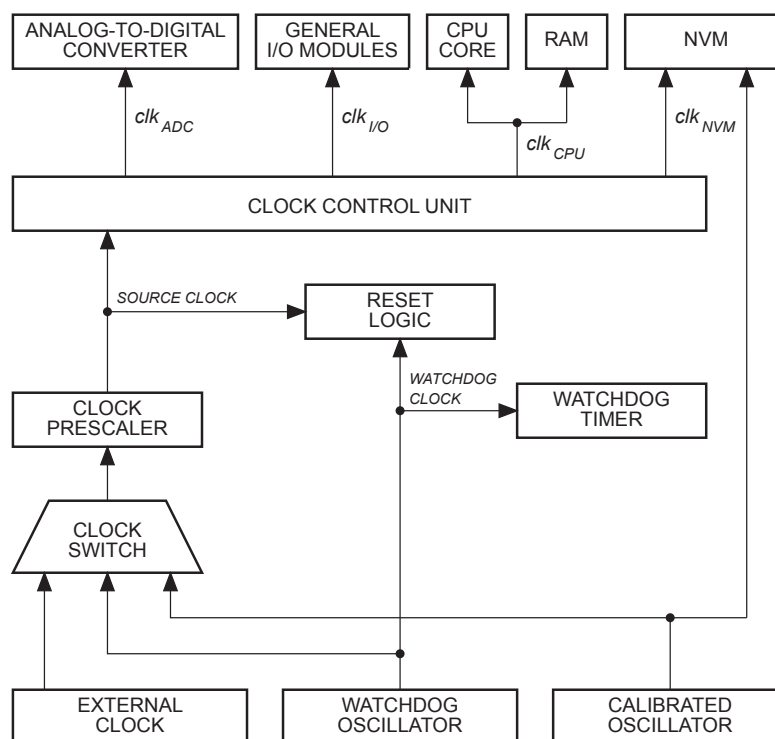
Figure 10-1. Clock Distribution
