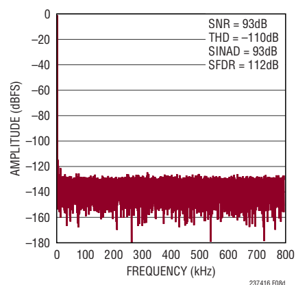
Figure 8d. 32k Point FFT f_{\text{SAMPL}} = 1.6\text{Msps} , f_{\text{IN}} = 1\text{kHz} for Circuit Shown in Figure 8a; Driven with Bipolar Inputs
