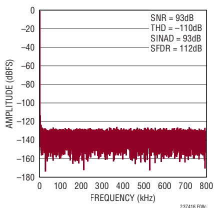
Figure 8c. 32k Point FFT f_{\text{SAMPL}} = 1.6\text{Msps} , f_{\text{IN}} = 1\text{kHz} for Circuit Shown in Figure 8a; Driven with Unipolar Inputs
