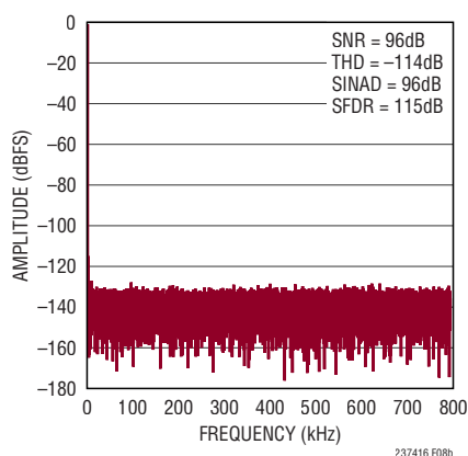
Figure 8b. 32k Point FFT f_{\text{SAMPL}} = 1.6\text{Msps} , f_{\text{IN}} = 1\text{kHz} for Circuit Shown in Figure 8a; Driven with Fully Differential Inputs
