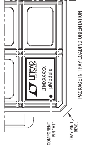
PACKAGE IN TRAY LOADING ORIENTATION
