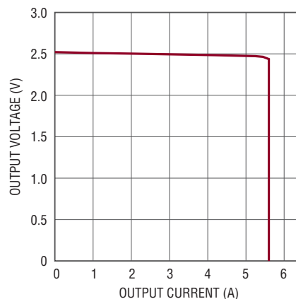
V_{OUT} vs I_{OUT} , 12V IN
