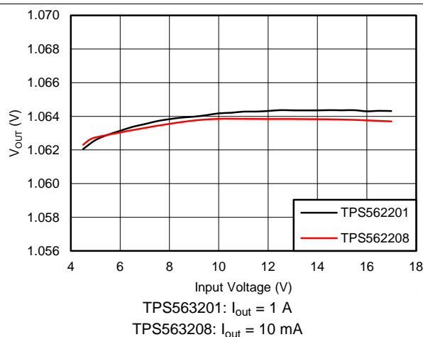
Figure 22. Line Regulation
