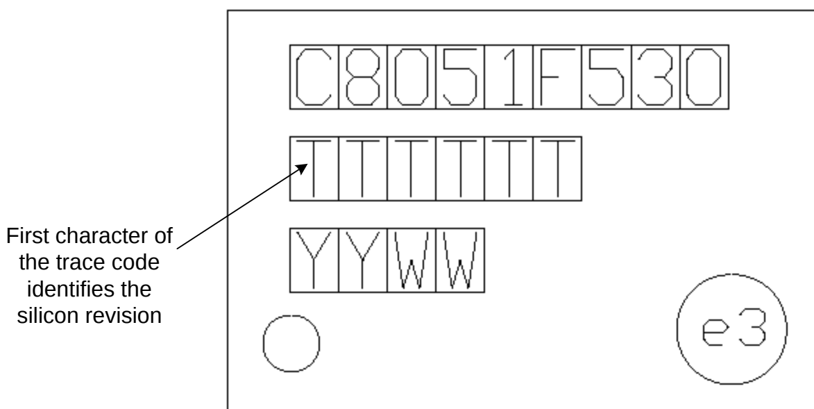
Figure 20.1. Device Package—TSSOP 20
