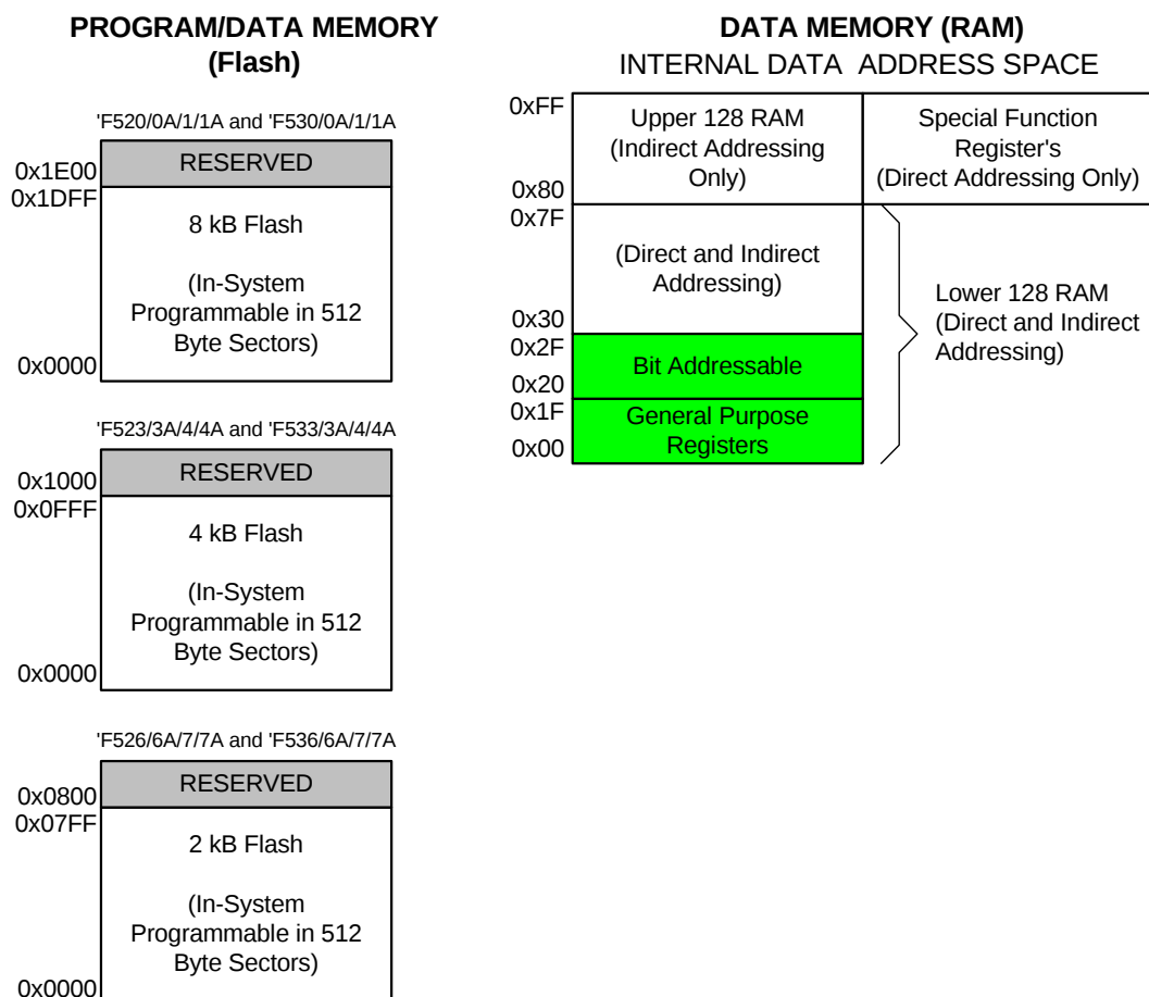
Figure 1.6. Memory Map
