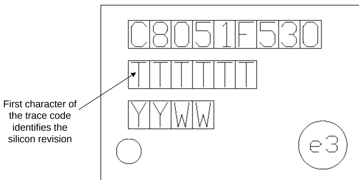
Figure 20.1. Device Package—TSSOP 20
