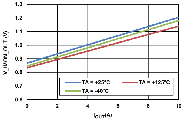
Figure 18. Output Current I_{OUT} (DC) vs IMON\_OUT Pin Voltage, R_{S\_OUT} = 4m\Omega , R_{IM\_OUT} = 43.2k
