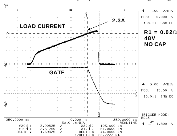
FIGURE 28. OVERCURRENT AT 2.3A
