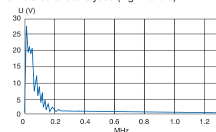
Fig. 3. Frequency spectrum
