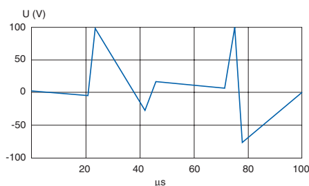
Fig. 2. Signal s(t)
