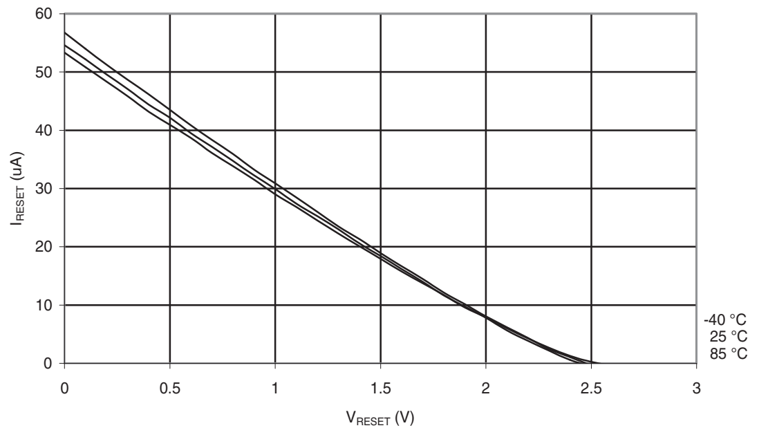
Figure 29-23. Reset Pull-up Resistor Current vs. Reset Pin Voltage ( V_{CC} = 2.7V )
