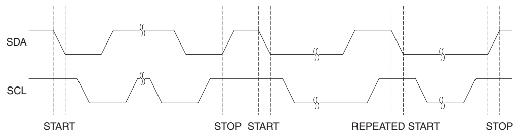
Figure 21-4. START, REPEATED START, and STOP Conditions
