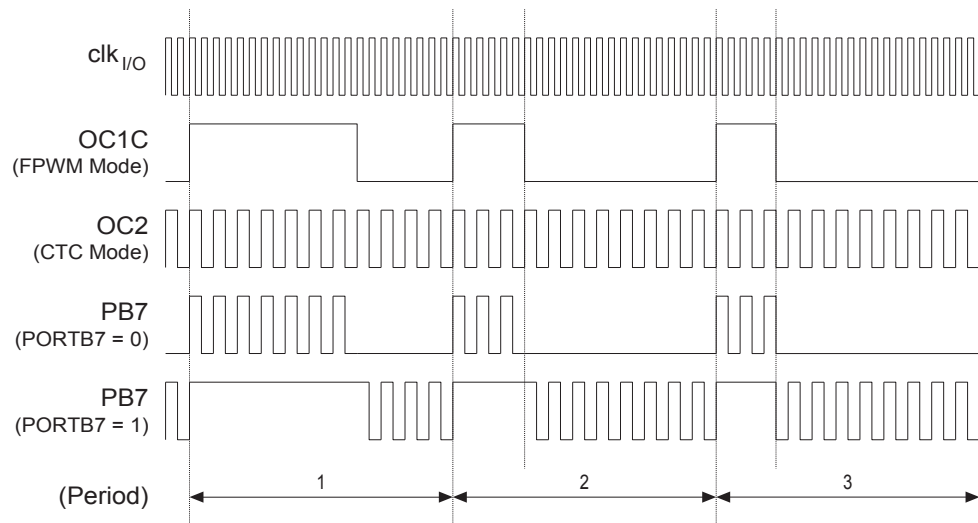
Figure 18-2. Output Compare Modulator, Timing Diagram
