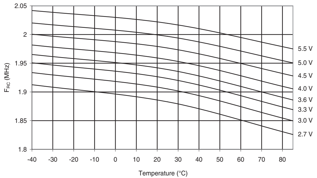
Figure 29-43. Calibrated 2 MHz RC Oscillator Frequency vs. Temperature
