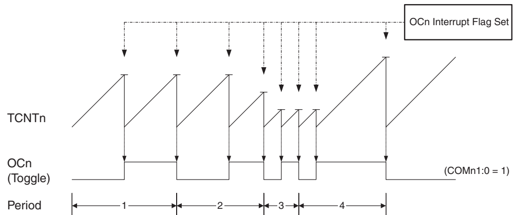
Figure 14-5. CTC Mode, Timing Diagram
