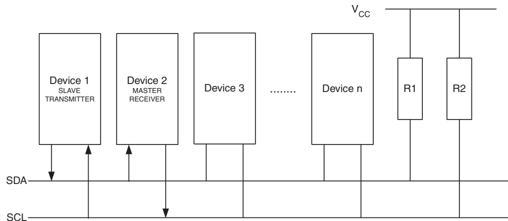
Figure 21-17. Data Transfer in Slave Transmitter Mode
