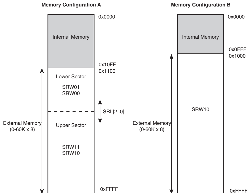
Figure 7-4. External Memory with Sector Select (1)
