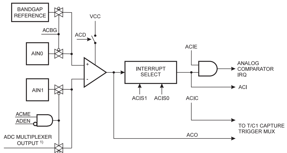
Figure 22-1. Analog Comparator Block Diagram (1)(2)
