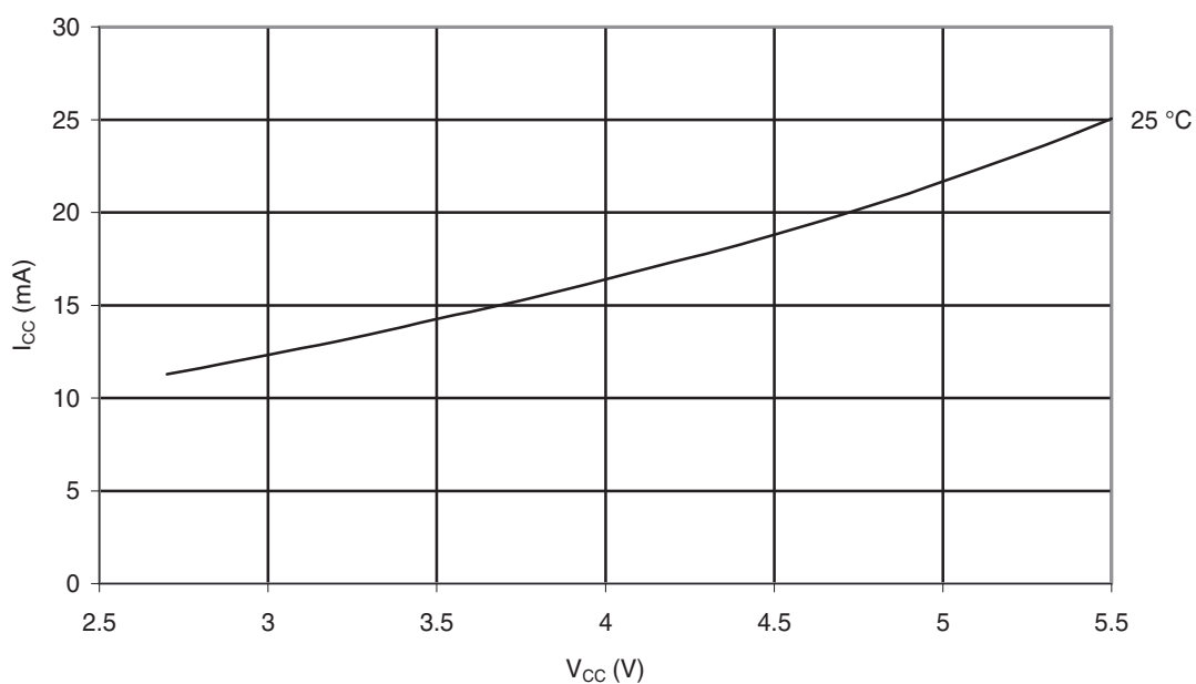
Figure 29-14. Idle Supply Current vs. V_{CC} (32 kHz External Oscillator)
