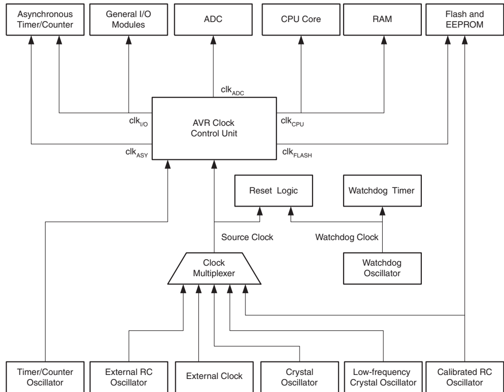
Figure 8-1. Clock Distribution
