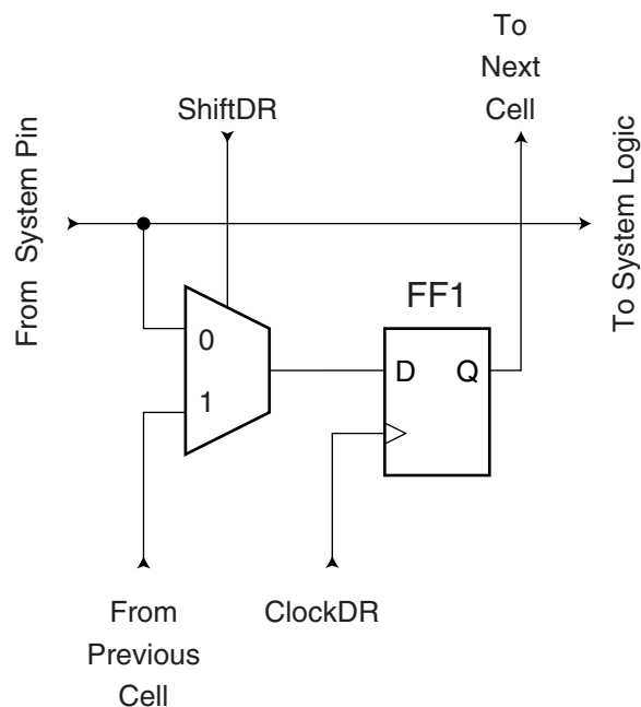
Figure 25-6. Observe-only Cell
