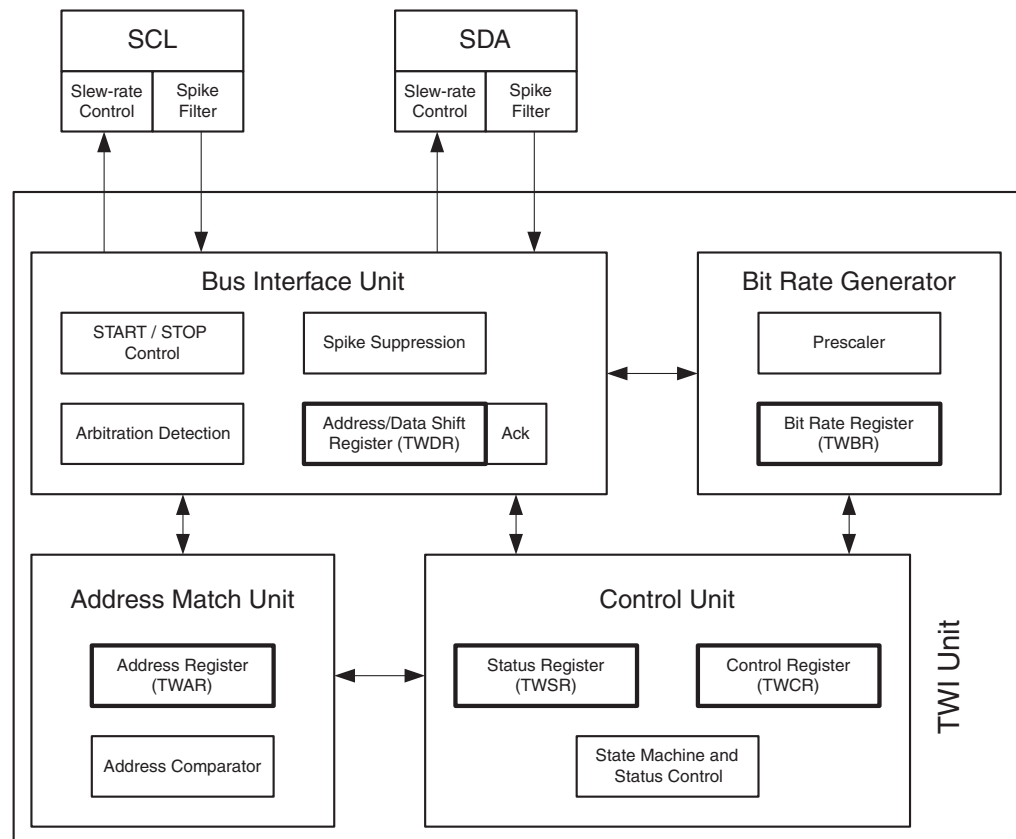
Figure 21-1. Overview of the TWI Module
