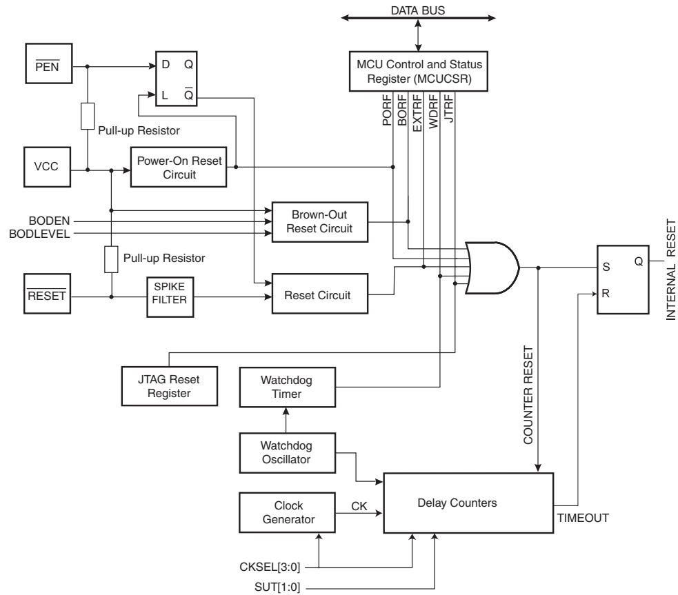
Figure 10-1. Reset Logic
