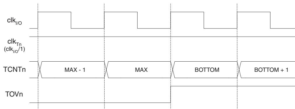
Figure 14-8. Timer/Counter Timing Diagram, no Prescaling
