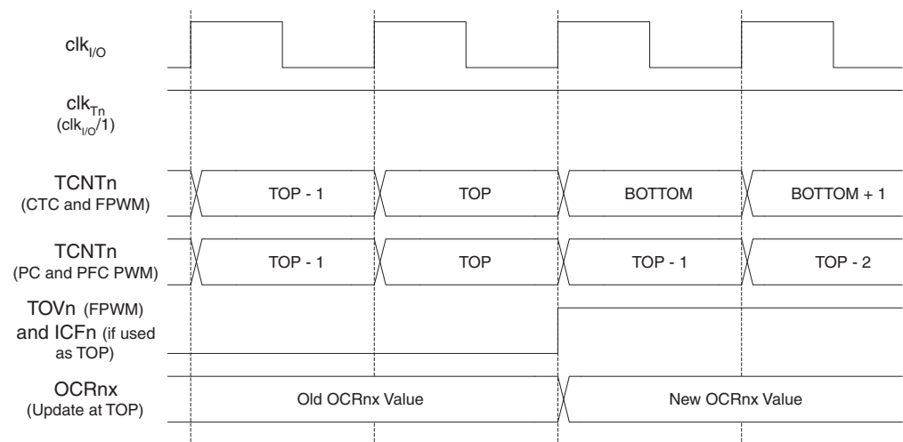
Figure 15-12. Timer/Counter Timing Diagram, no Prescaling
