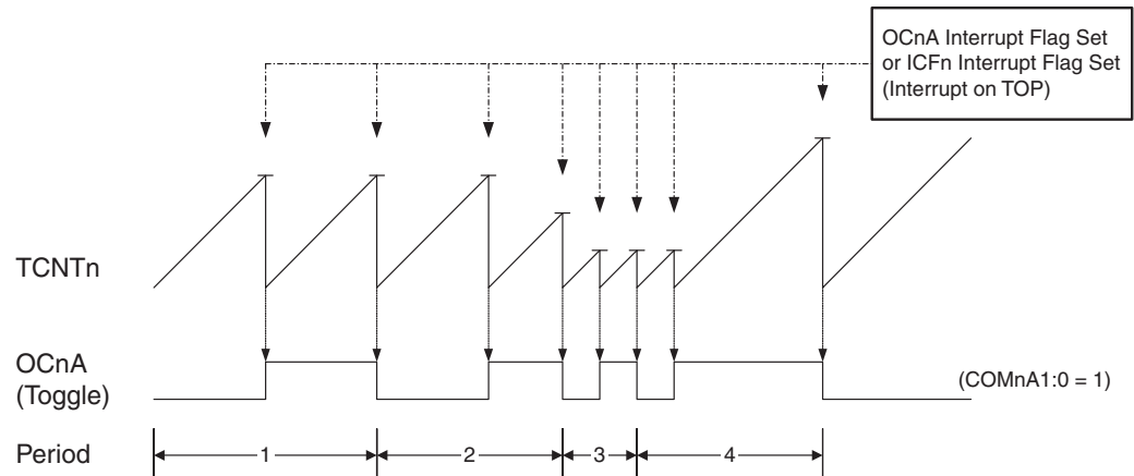
Figure 15-6. CTC Mode, Timing Diagram
