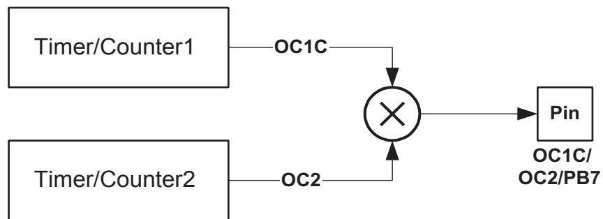
Figure 18-1. Output Compare Modulator, Block Diagram
