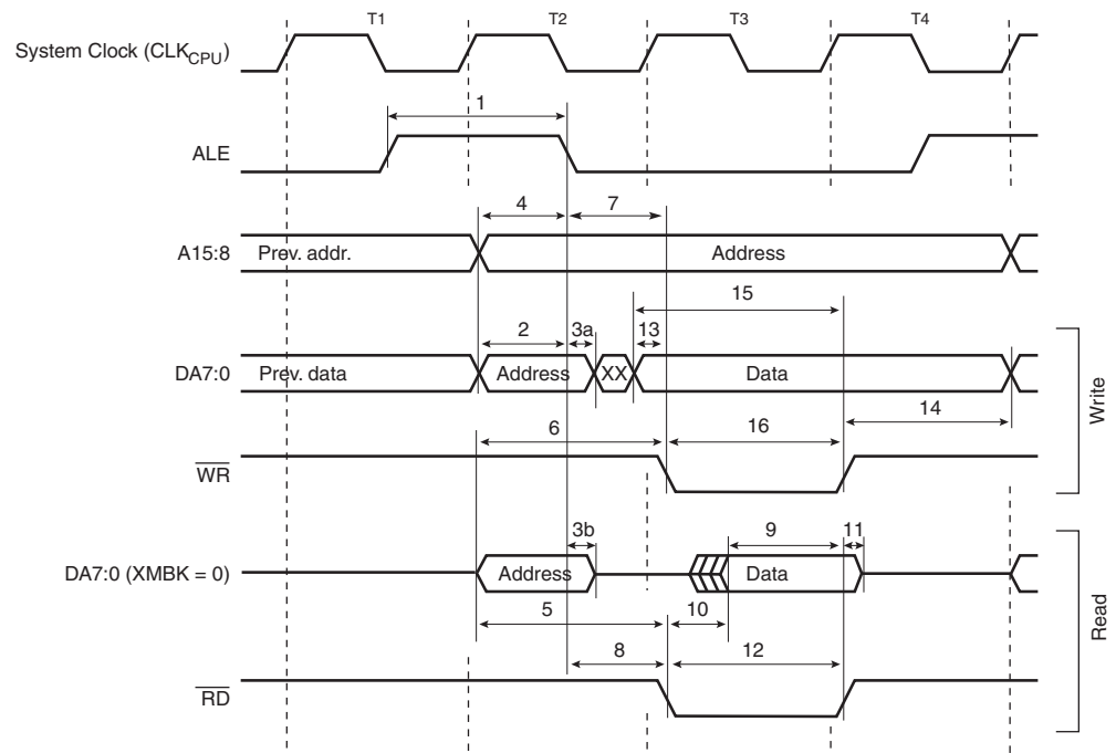
Figure 28-6. External Memory Timing (SRWn1 = 0, SRWn0 = 0)
