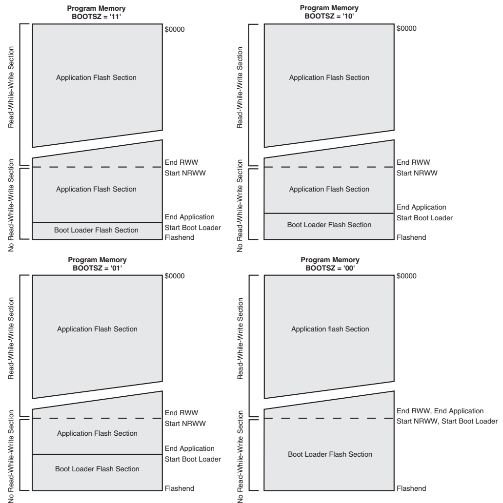
Figure 26-2. Memory Sections (1)
