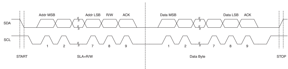
Figure 21-7. Typical Data Transmission
