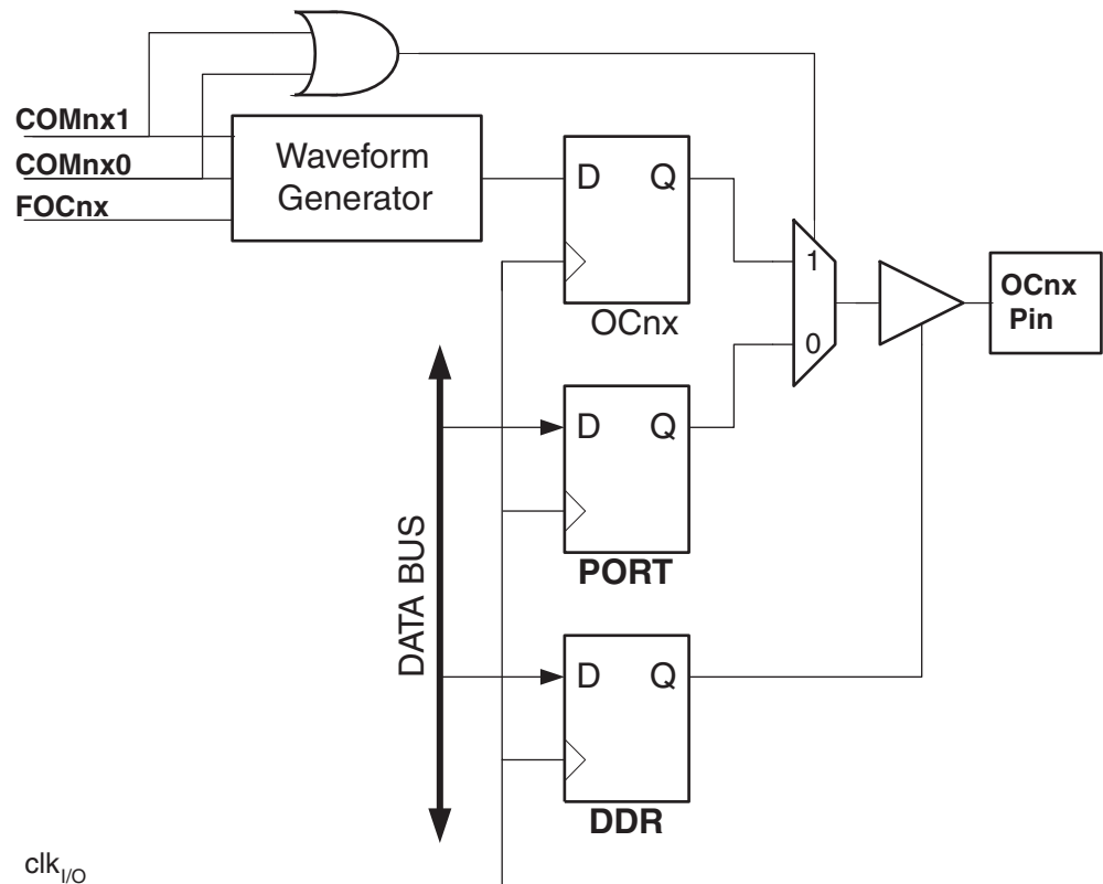
Figure 15-5. Compare Match Output Unit, Schematic
