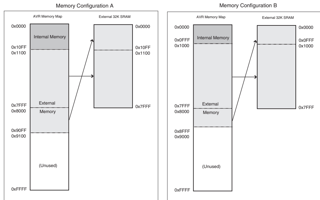
Figure 7-10. Address Map with 32 KB External Memory
