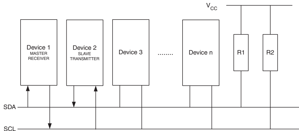
Figure 21-13. Data Transfer in Master Receiver Mode
