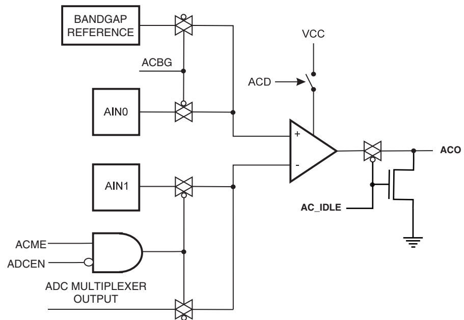
Figure 25-8. Analog Comparator
