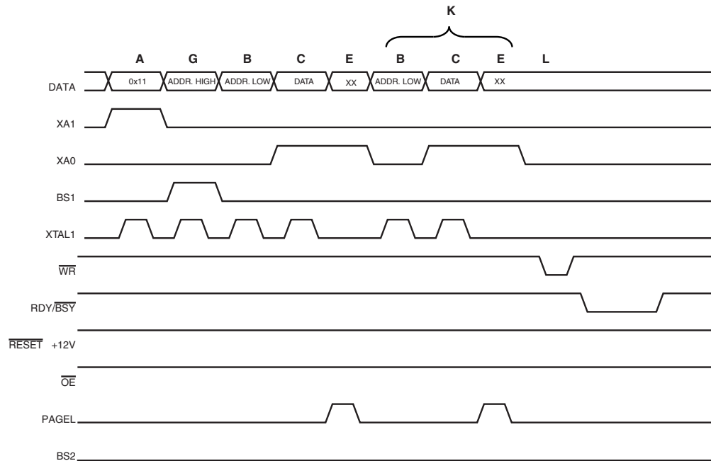
Figure 27-4. Programming the EEPROM Waveforms
