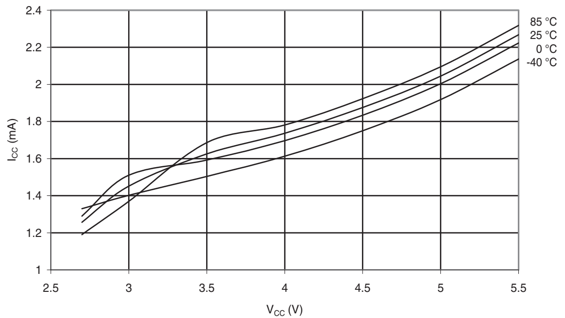
Figure 29-3. Active Supply Current vs. V_{CC} (Internal RC Oscillator, 1 MHz)
