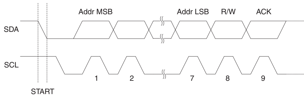
Figure 21-5. Address Packet Format
