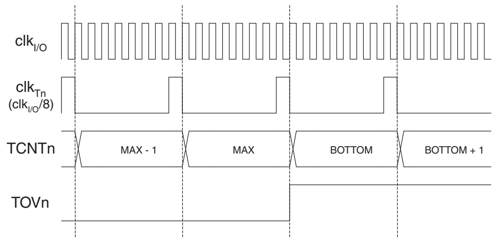
Figure 17-9. Timer/Counter Timing Diagram, with Prescaler ( f_{\text{clk\_I/O}}/8 )
