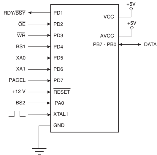
Figure 27-1. Parallel Programming
