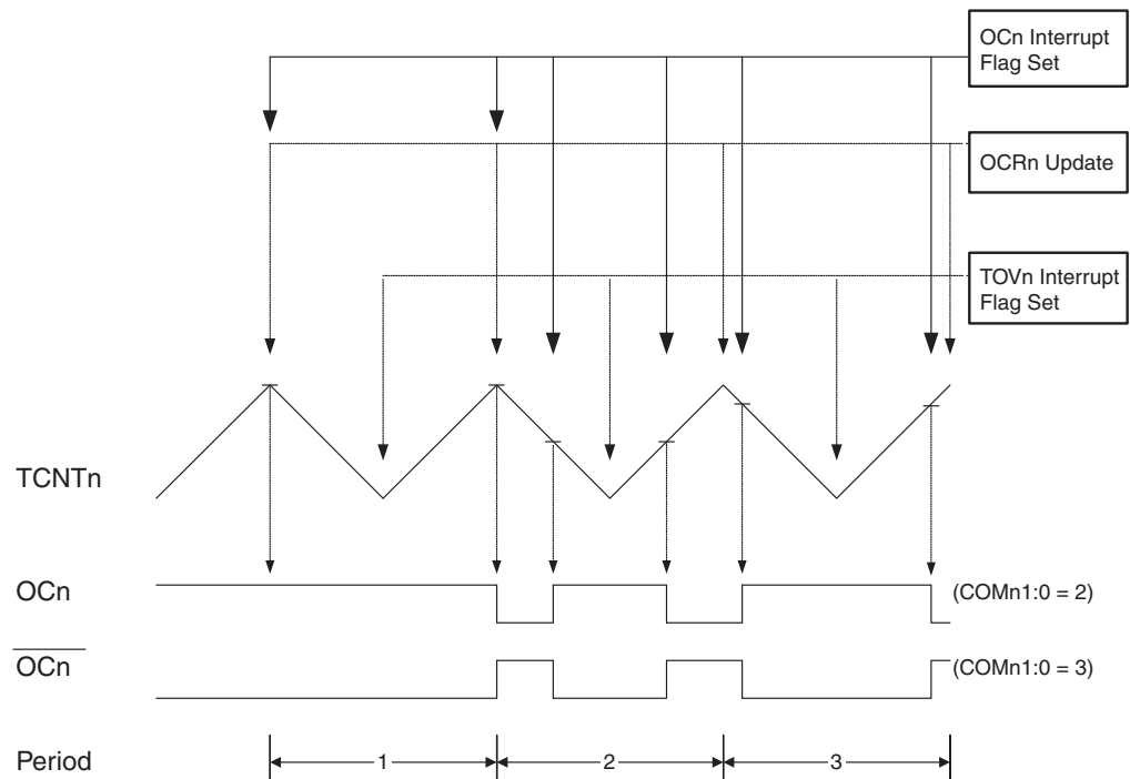
Figure 17-7. Phase Correct PWM Mode, Timing Diagram
