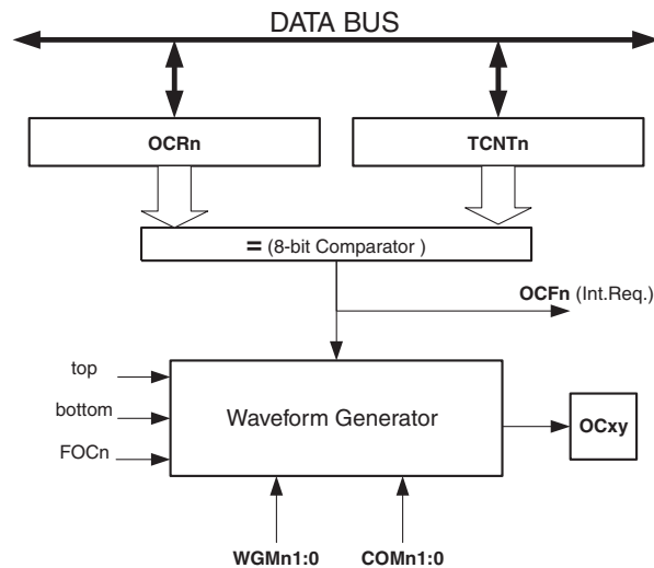
Figure 14-3. Output Compare Unit, Block Diagram
