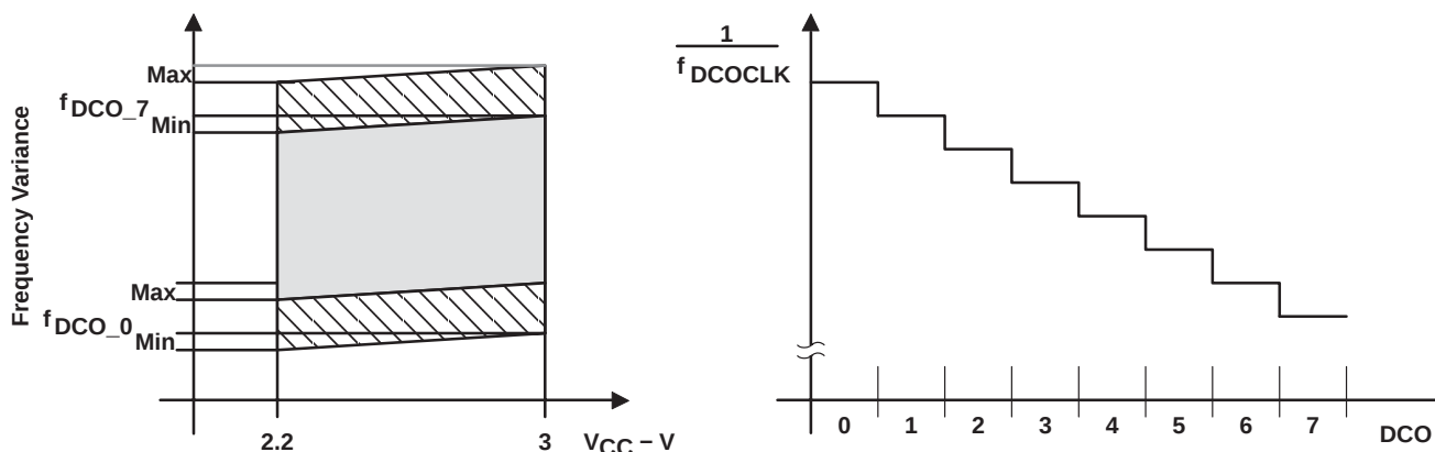
Figure 12. DCO Characteristics
