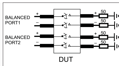
Diff. Near End Xtalk Test Circuit
