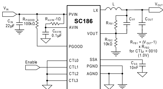
Figure 2 — Output Voltage Programming
