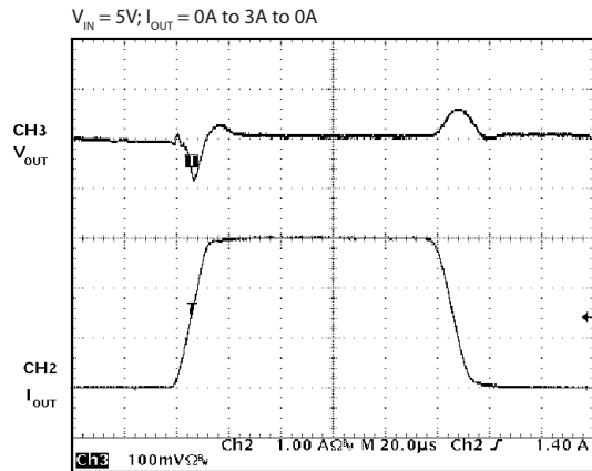
Transient Response ( V_{OUT}=1.5\text{V} , I_{STEP}=3\text{A} )
