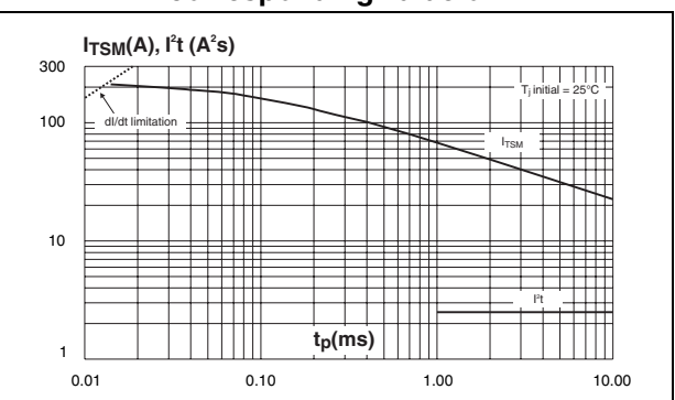
Figure 10. Non repetitive surge peak on state current for a sinusoidal pulse and corresponding value of I²t
