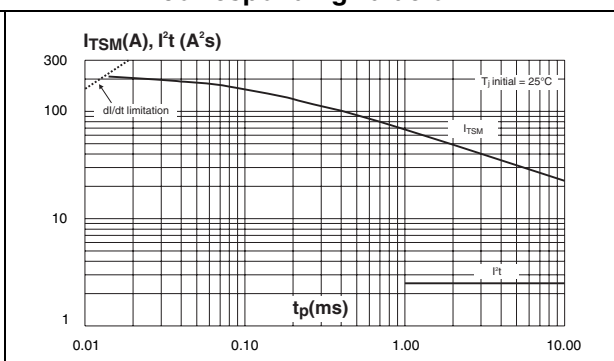
Figure 10. Non repetitive surge peak on state current for a sinusoidal pulse and corresponding value of I²t
