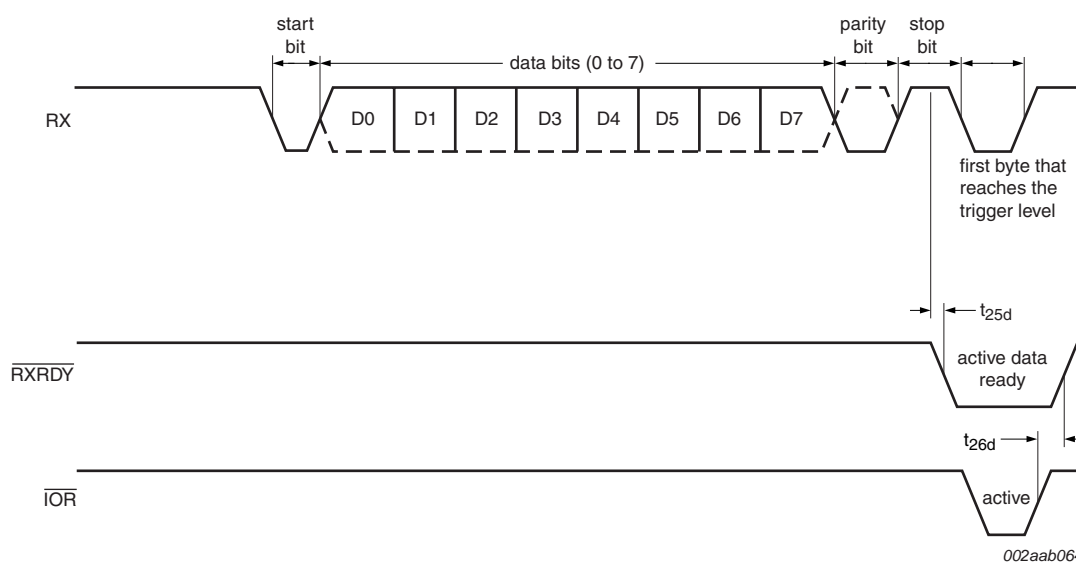
Fig 26. Receive ready timing in FIFO mode
