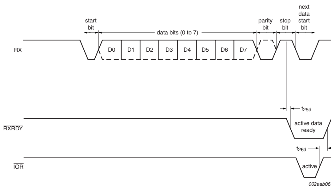
Fig 25. Receive ready timing in non-FIFO mode
