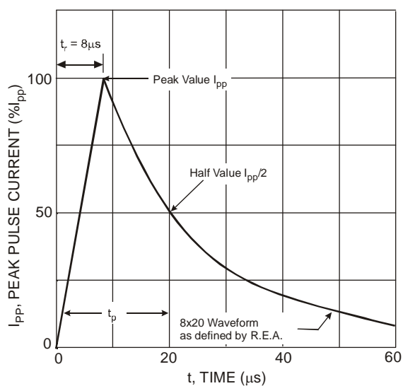
Figure 3 Pulse Waveform
