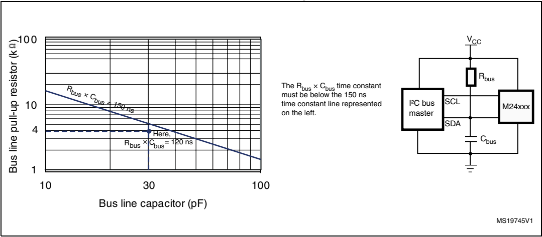
Figure 13. Maximum R_{bus} value versus bus parasitic capacitance C_{bus} ) for an I 2 C bus at maximum frequency f_C = 1 MHz
