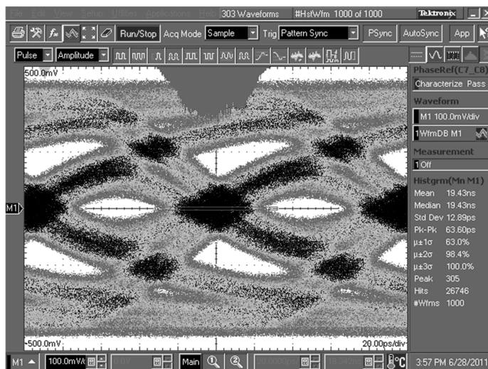
Figure 22. 10" of 4 mil FR4 Without De-Emphasis
