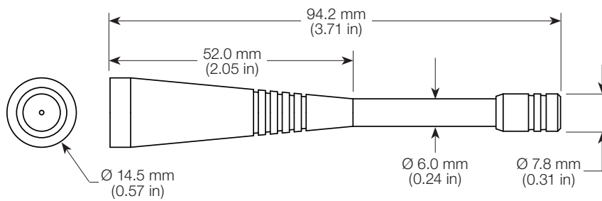
Figure 7. CW LTE Band 14 Antenna Dimensions
