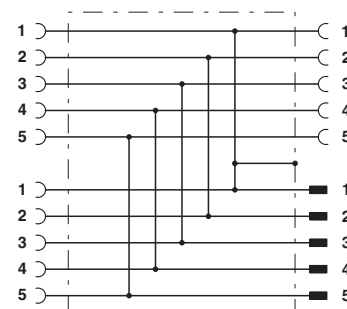
Contact assignment of the M12 H distributor
