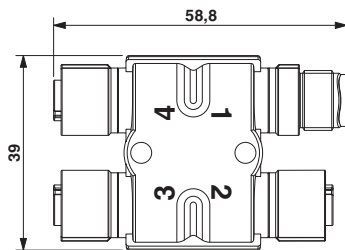
H distributor dimensional drawing
