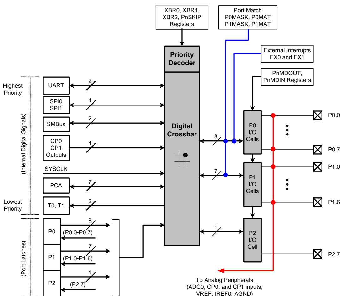
Figure 1.5. Port I/O Functional Block Diagram
