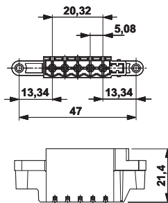
Dimensioned drawing
