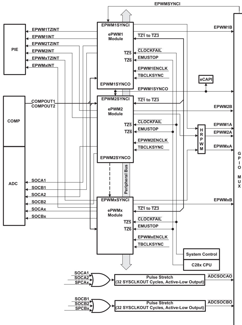
Figure 4-8. ePWM
