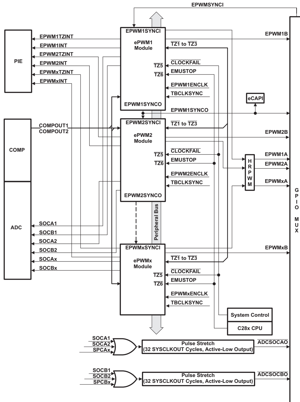
Figure 4-8. ePWM
