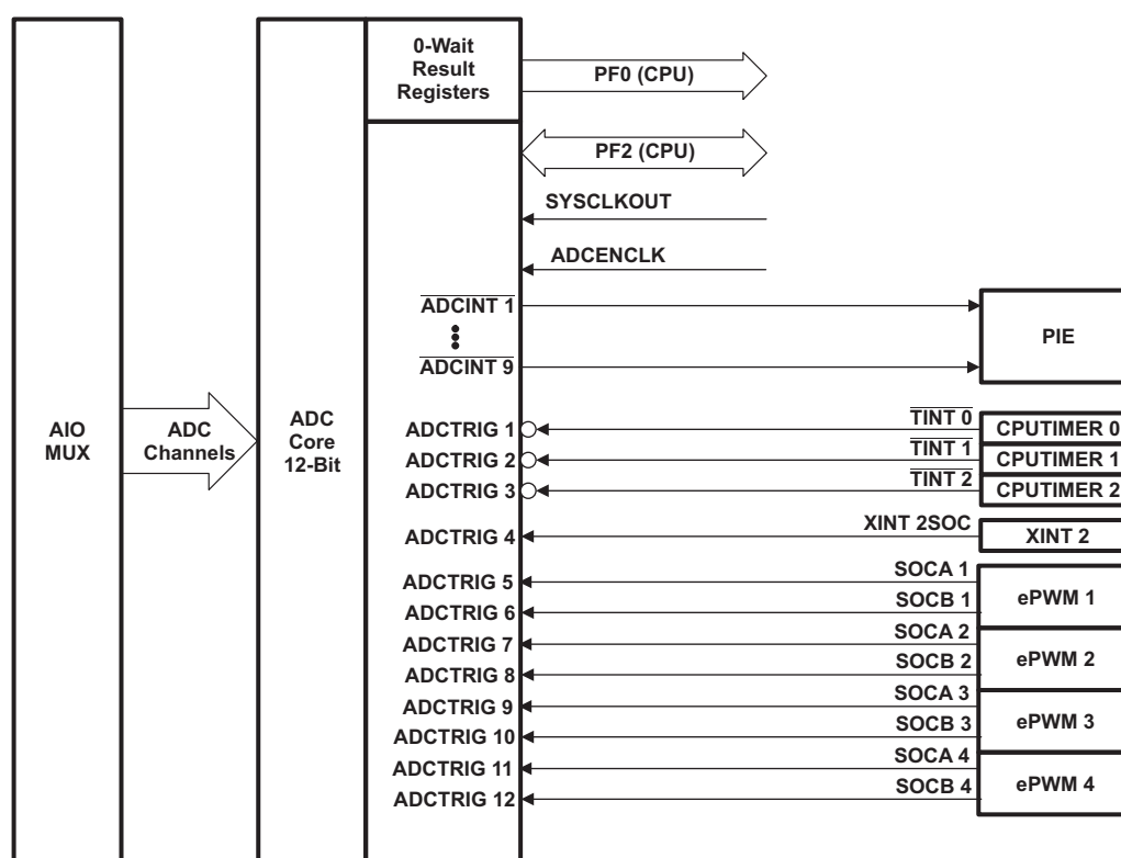
Figure 4-2. ADC Connections
