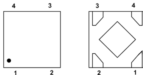
Top View X2-DFN1010-4 Bottom View
