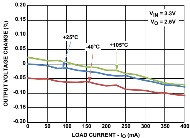
FIGURE 4. LOAD REGULATION
