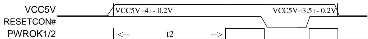
Figure 11-12. PWROK1/2 Timings
