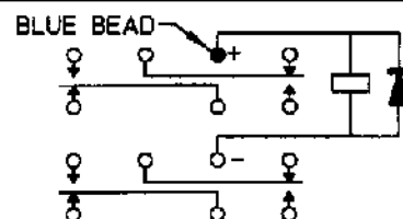
TERMINAL VIEW
