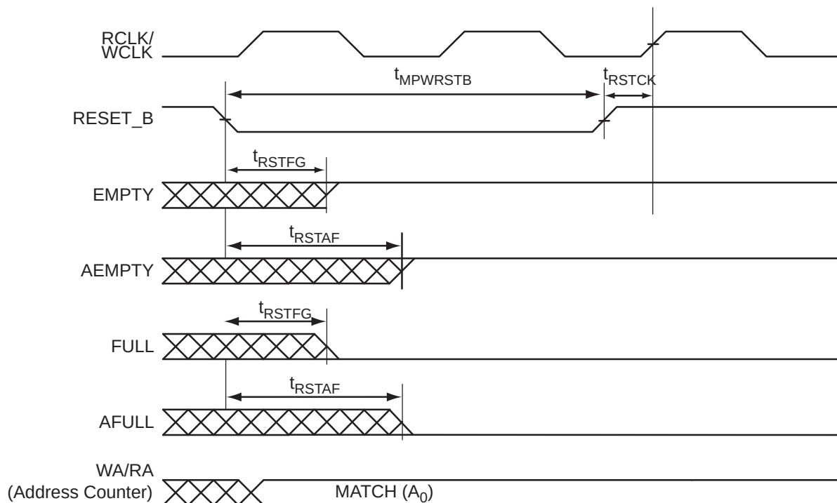
Figure 2-51 • FIFO Reset
