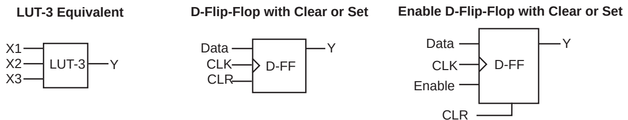
Figure 1-4 • VersaTile Configurations
