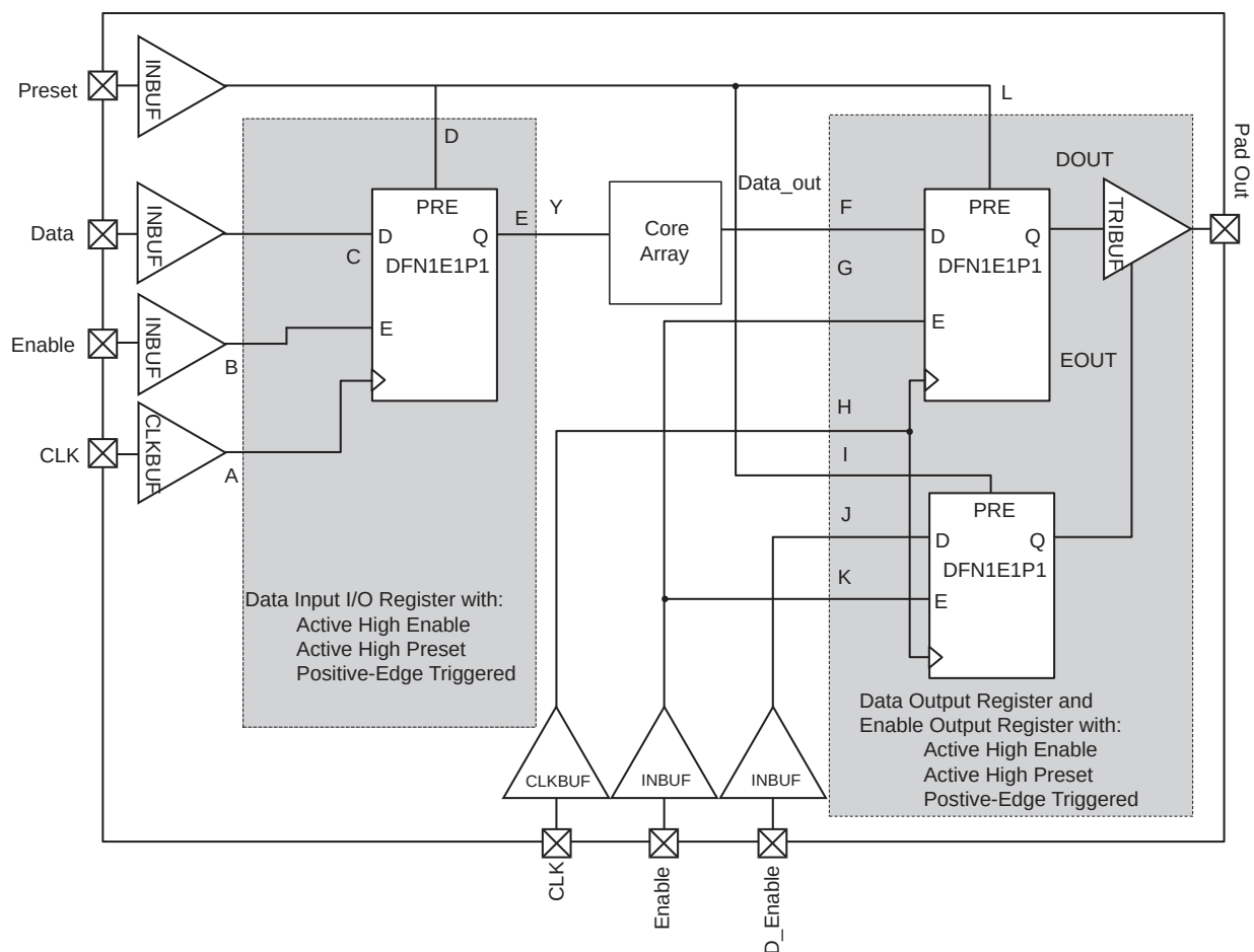
Figure 2-29 • Timing Model of Registered I/O Buffers with Synchronous Enable and Asynchronous Preset
