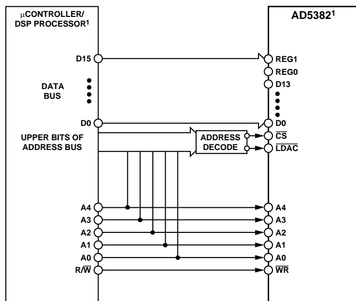
Figure 34. AD5382-to-Parallel Interface
