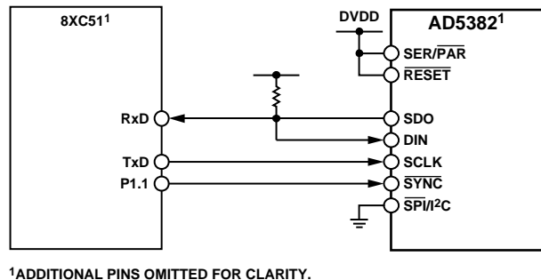
Figure 36. AD5382-to-8051 Interface
