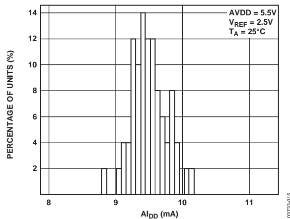
Figure 14. AIDD Histogram
