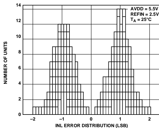
Figure 18. INL Error Distribution
