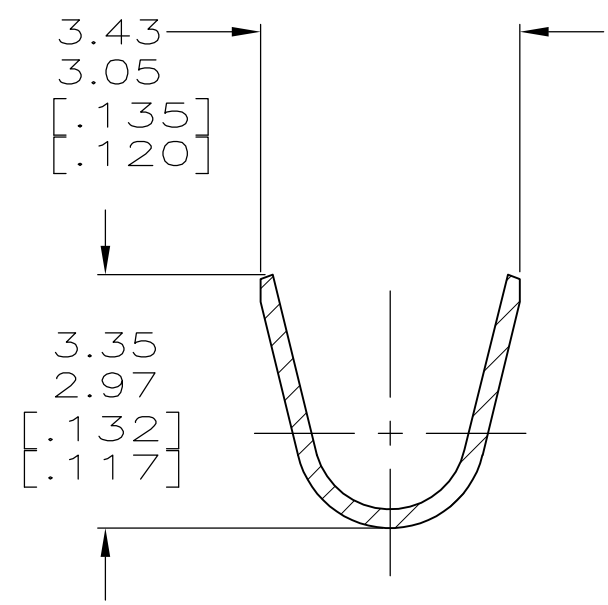
SECTION A-A INSULATION RANGE .095-.045 DIA
