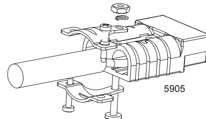
Bolt on bundled conductors.
