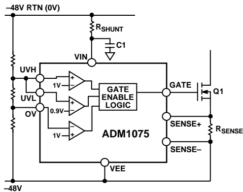
Figure 51. Undervoltage and Overvoltage Supply Monitoring
