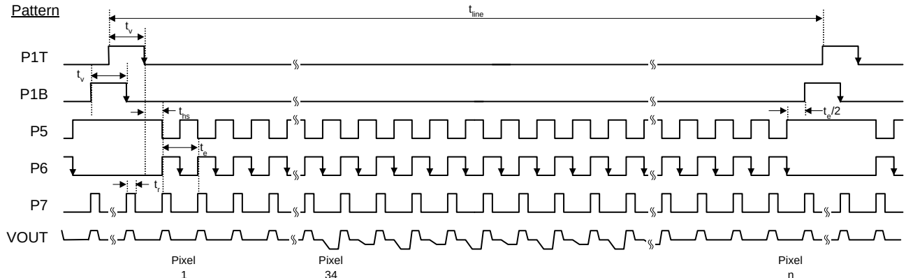
Figure 25. Line and Pixel Timing
