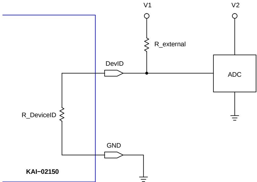
Figure 23. Device Identification Recommended Circuit
