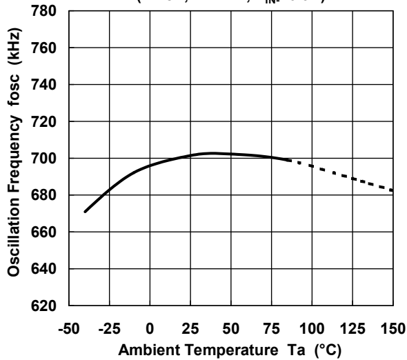
Oscillation Frequency vs Temperature (B ver., V^+=12V , V_{IN}=0.9V )
