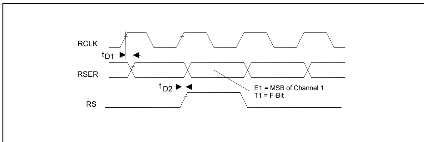
Figure 19-10. Receive Timing, T1/E1
