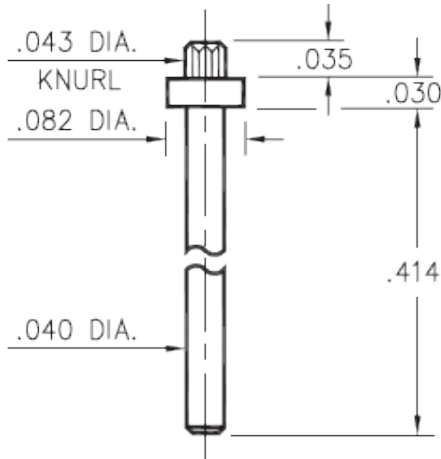
4526-0-00-XX-00-00-03-0 Press-fit in .040 mounting hole
