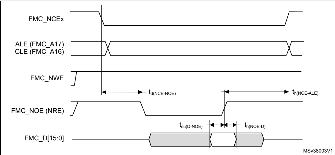
Figure 43. NAND controller waveforms for read access
