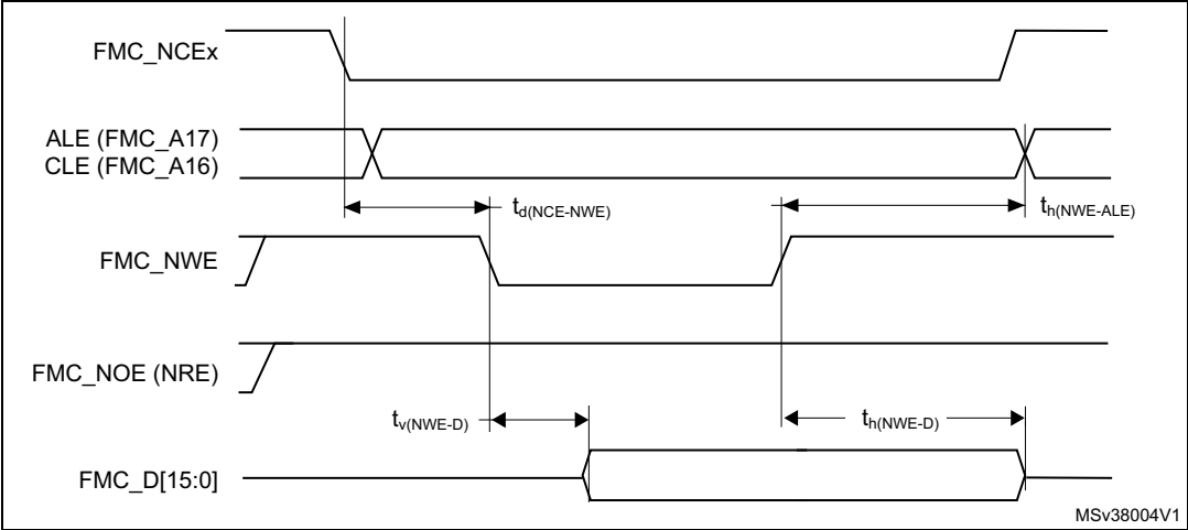
Figure 44. NAND controller waveforms for write access
