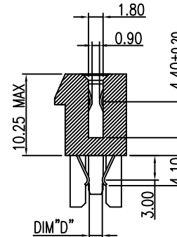
SECTION P-P
