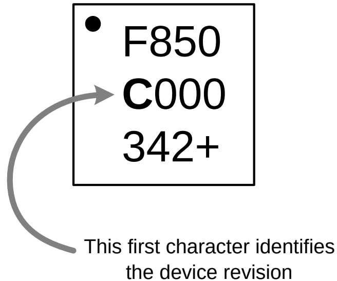
Figure 28.2. QFN-20 Package Revision Marking
