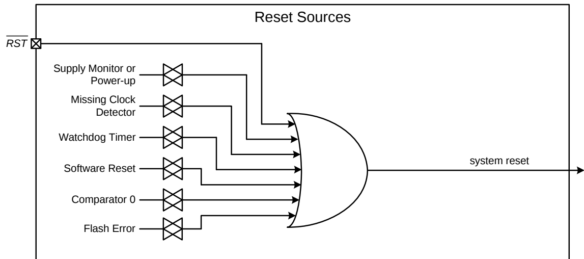
Figure 22.1. Reset Sources
