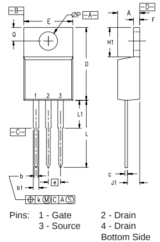
TO-220 AD Dimensions
