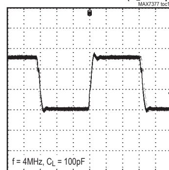
CLOCK OUTPUT WAVEFORM (C L = 100pF)
