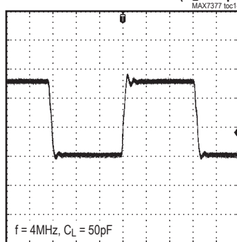
CLOCK OUTPUT WAVEFORM (C L = 50pF)
